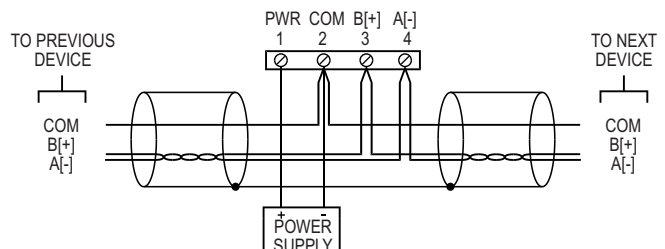
Figure 3: Local power supply wiring
