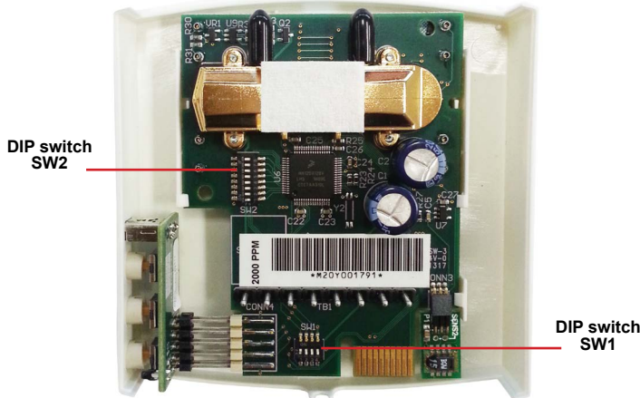
Figure 6: Internal view of transmitter
