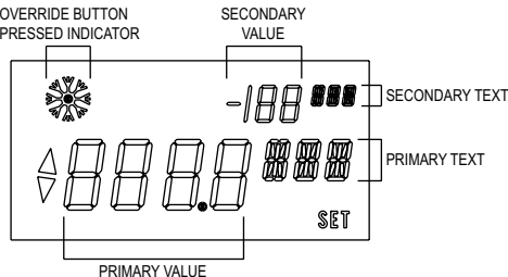
Figure 7: Display layout
